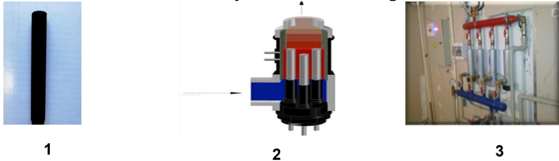
Fig. 1. 1 - external appearance of electrode, 2 - electric boiler, 3 - heated system
