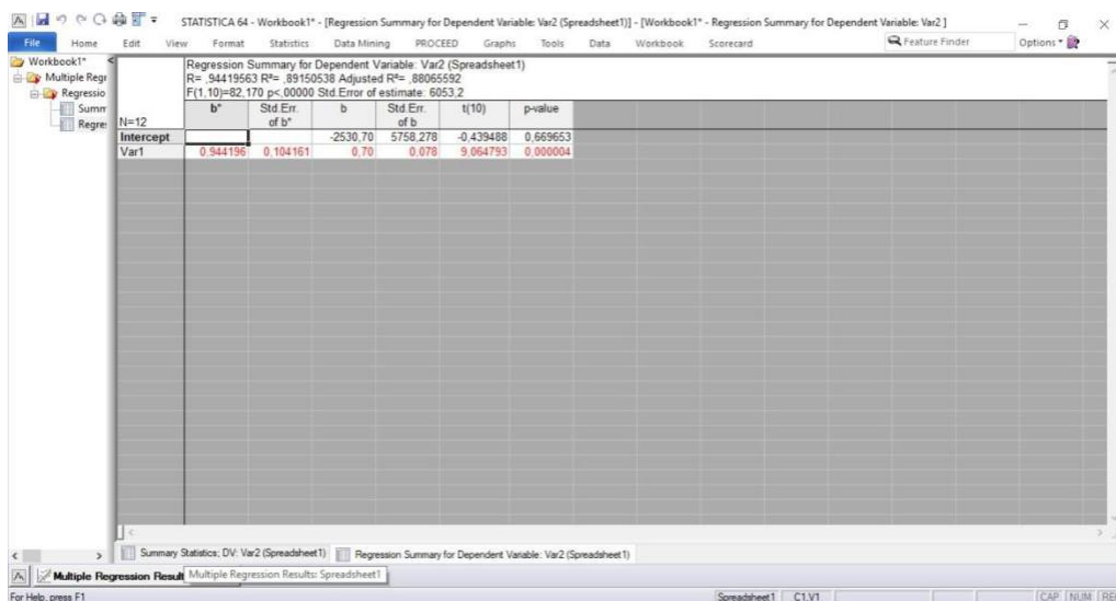
Figure 2. Regression results
