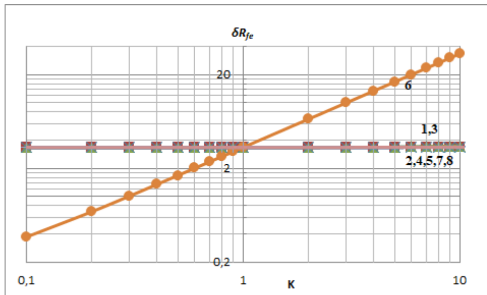
Figure 7. Dependence of the equivalent steel loss resistance determination error change.
