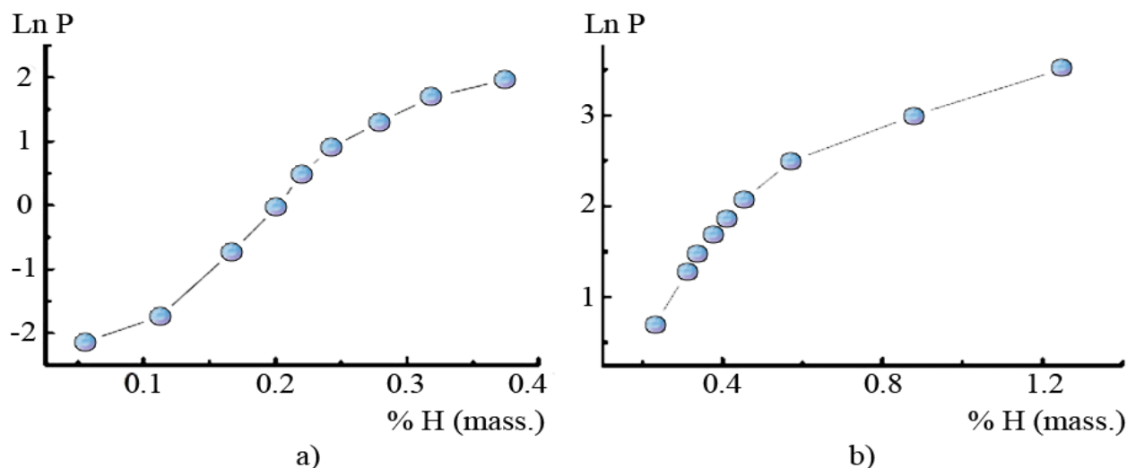
Figure 1 - Equilibrium hydrogen desorption curves for \text{ZrNi}_{1.2}\text{Mn}_{0.5}\text{Cr}_{0.2}\text{V}_{0.1} alloy electrodes at 20°C (a) and 100°C (b) obtained in a gaseous medium on the activated surface of the alloy.
