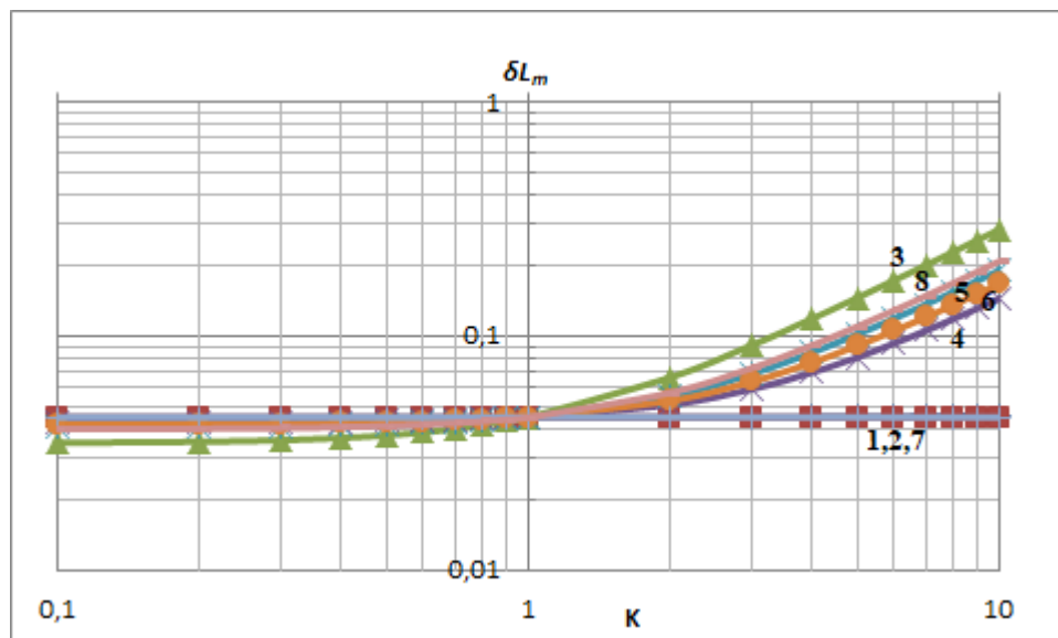
Figure 4. Dependence of the magnetization inductance determination error change.
