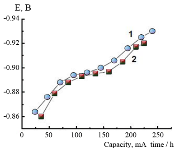
Figure 2 - Equilibrium hydrogen desorption curves for electrodes made of \text{ZrNi}_{1.2}\text{Mn}_{0.5}\text{Cr}_{0.2}\text{V}_{0.1} (1) and \text{ZrNi}_{1.2}\text{Mn}_{0.5}\text{Cr}_{0.2}\text{Al}_{0.1} (2) alloys obtained electrochemically on the activated electrode surface.
