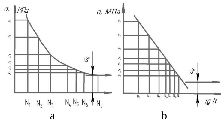
Fig. 2 – Fatigue curves in natural (a) and semilogarithmic coordinates (b)
