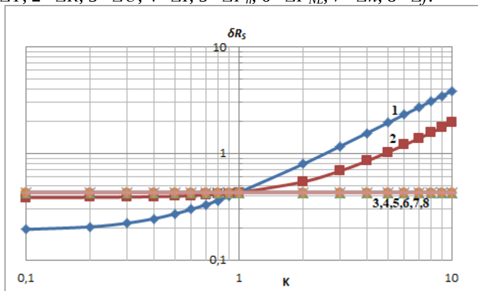
Figure 2. Dependence of the stator resistance determination error change.
