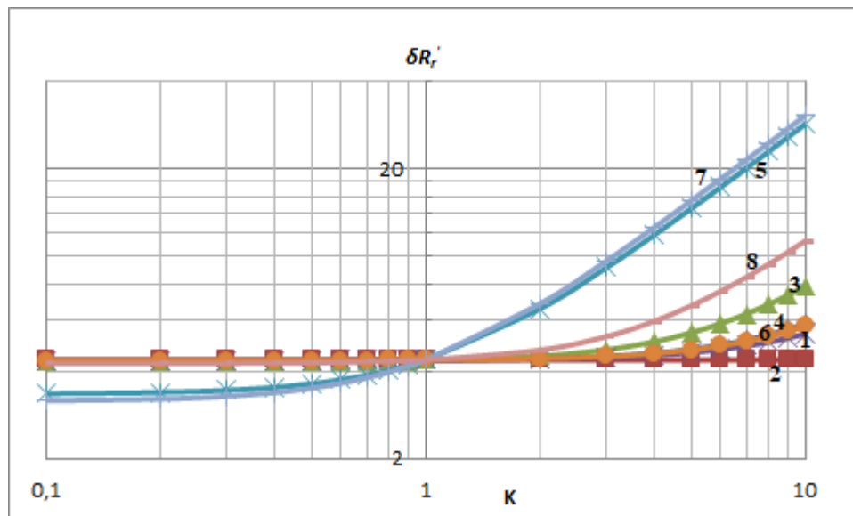
Figure 3. Dependence of rotor resistance determination error change.
