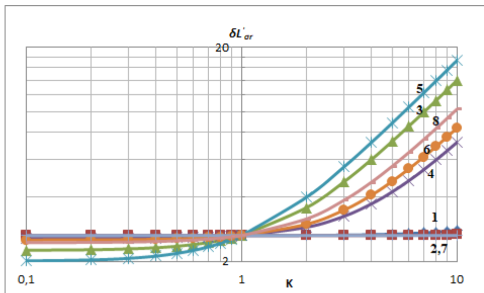
Figure 6. Dependence of the rotor scattering inductance determination error change.
