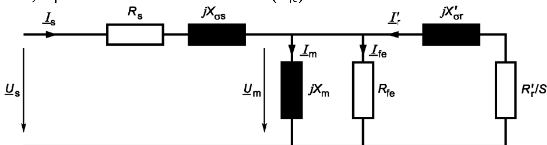
Figure 1. T-shaped phase replacement circuit of an induction electric machine.
