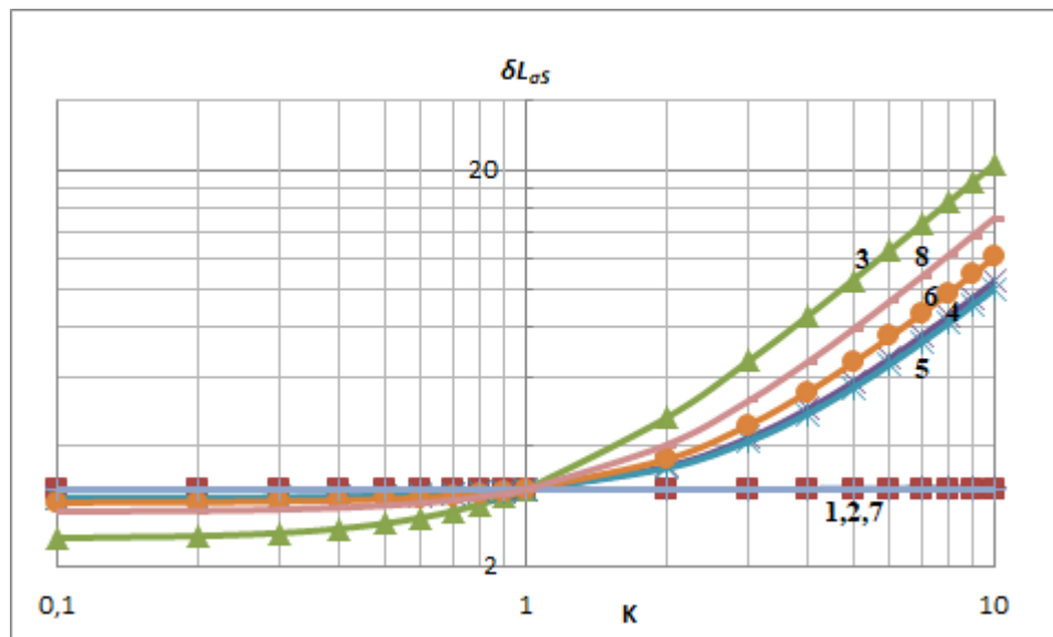
Figure 5. Dependence of the stator scattering inductance determination error change.
