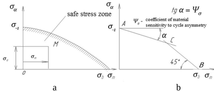
Fig. 3 – Diagram of boundary amplitudes in natural (a) and schematized (b) forms
