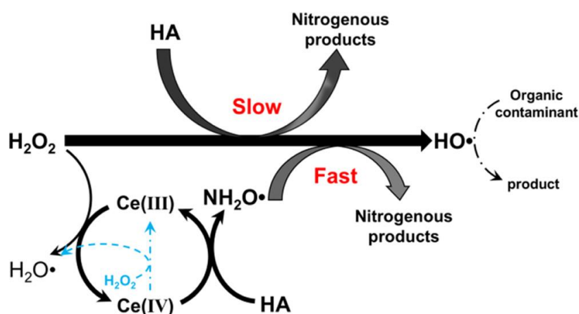
Figure 6. The proposed mechanism of organic contaminant degradation in Ce(IV)/H 2 O 2 /hydroxylamine system [101] under the terms of the Creative Commons CC BY license
