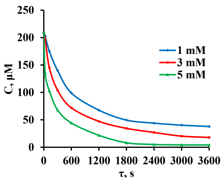
Figure 9. Influence of the initial dose of sodium percarbonate (in mM) in the reaction medium on the kinetics of oxidative degradation of Rhodamine B (conditions: V = 200 \text{ mL} ; C_0(\text{C}_{28}\text{H}_{31}\text{ClN}_2\text{O}_3) = 209 \mu\text{M} ; catalyst content ( \text{MgMn}_2\text{O}_4 spinel nanoparticles) – 1.0 \text{ g/L} ; \text{pH} = 3 ; T = 298 \text{ K} ; specific power of ultrasonic treatment – 51 \text{ W/L} ) [made by the authors]
